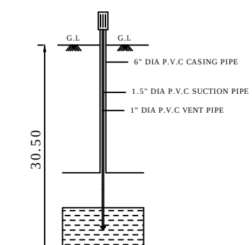
BORE WELL
