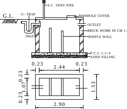
SEPTIC TANK DETAIL
