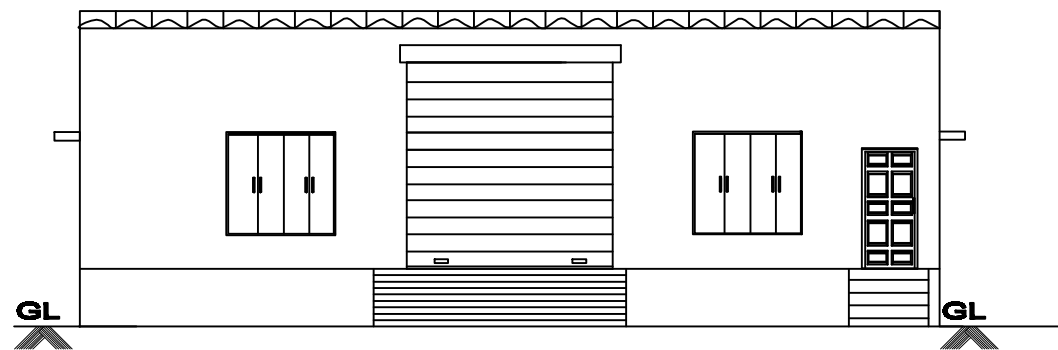
FRONT ELEVATION
