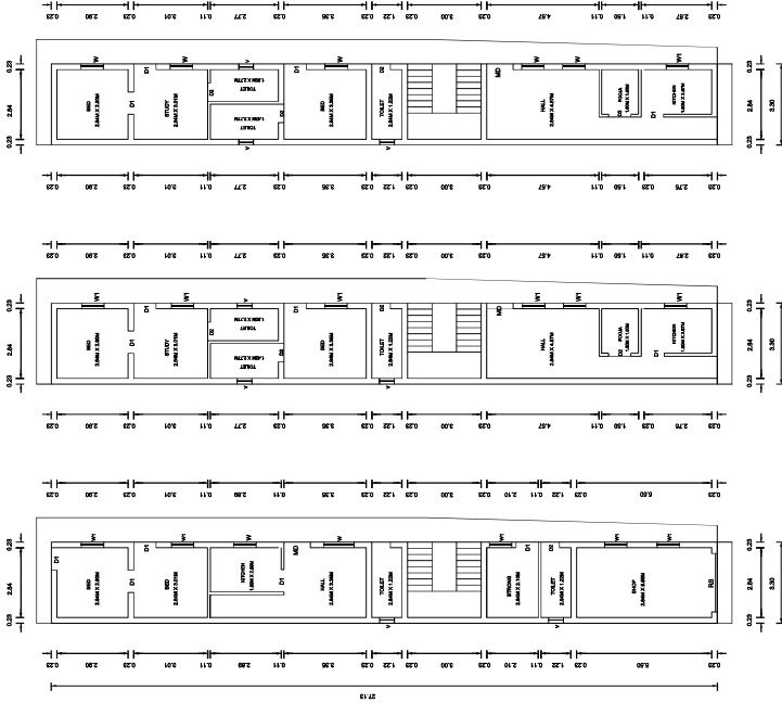
GROUND FLOOR PLAN ( COMMERCIAL & RESIDENTIAL )
