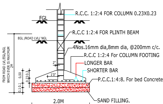
FOUNDATION DETAIL
