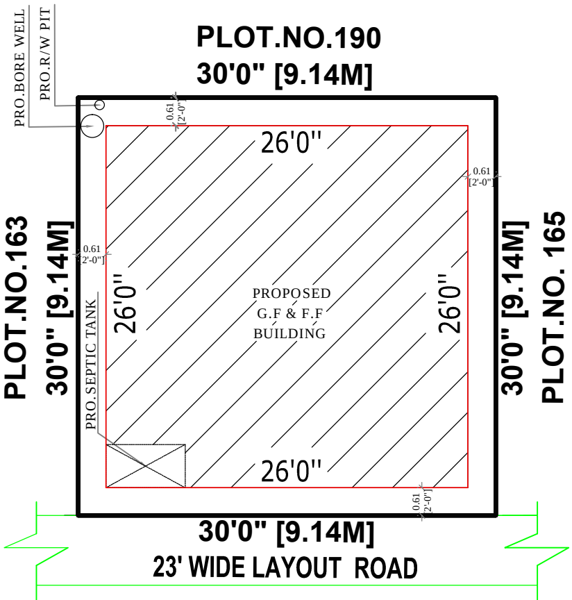
SITE PLAN
