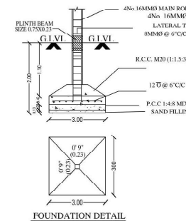
FOUNDATION DETAIL
