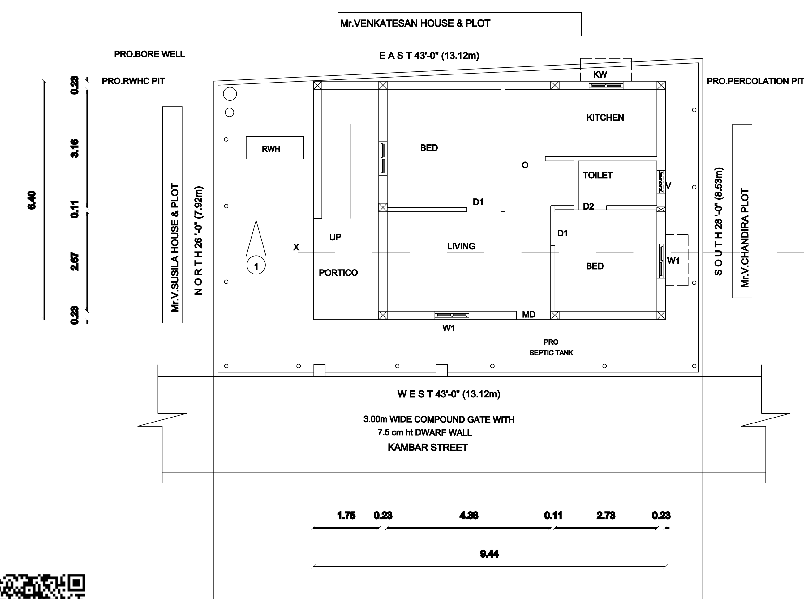
SITE CUM GROUND FLOOR PLAN
