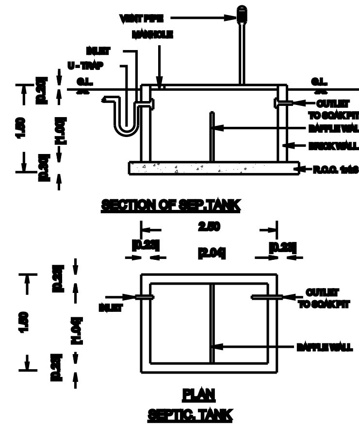
SECTION OF SEPTIC TANK
