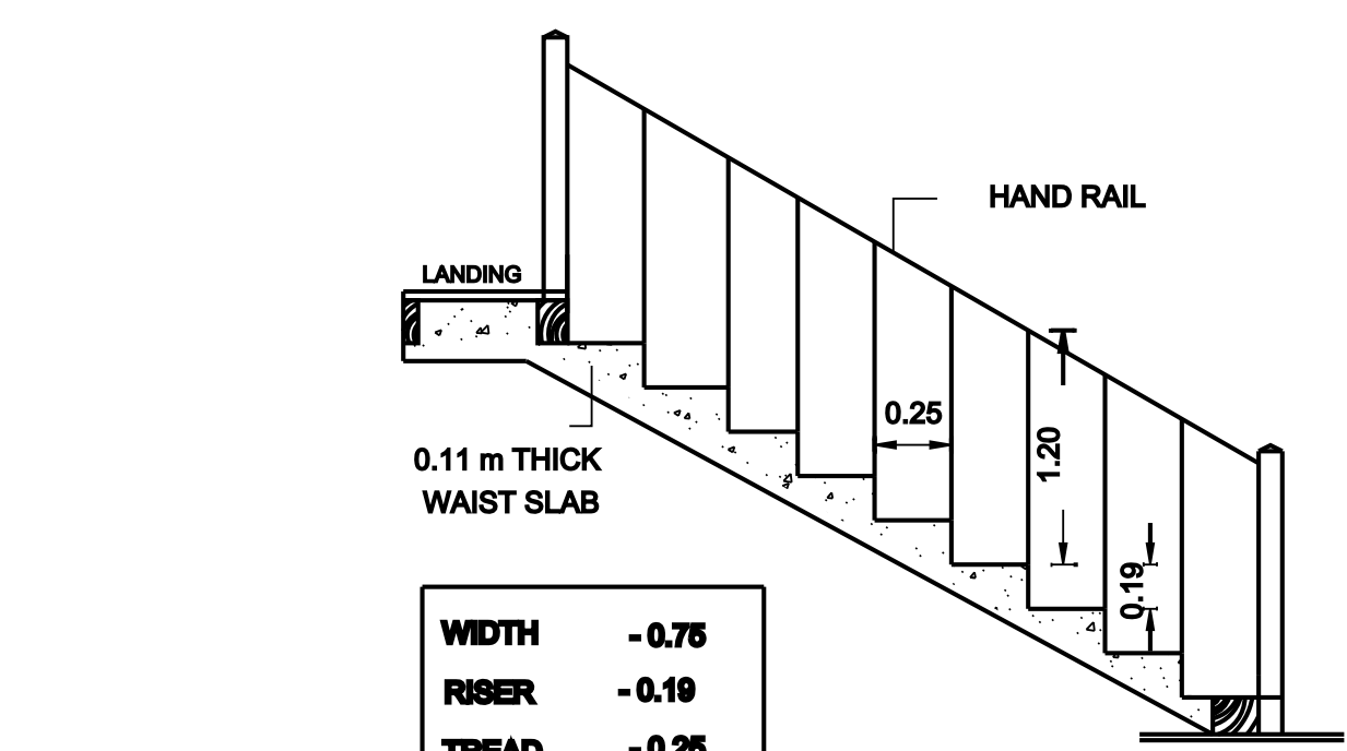
STAIRCASE DETAIL
