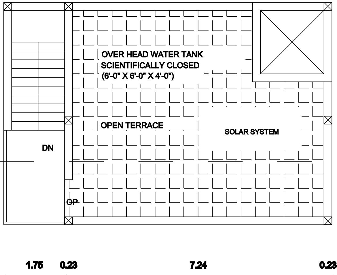
PRO.TERRACE FLOOR PLAN
