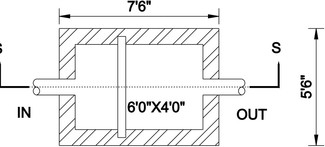
PLAN SEPTIC TANK NOT TO SCALE
