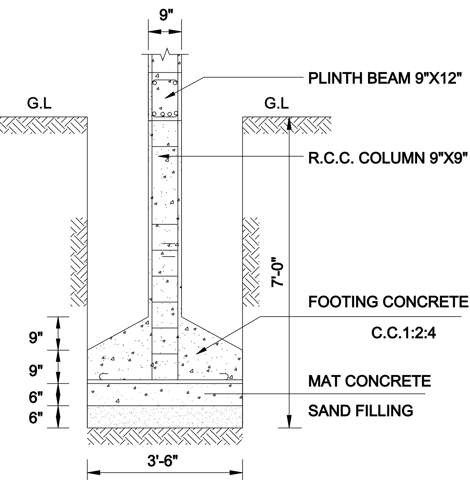
FOUNDATION DETAILS NOT TO SCALE
