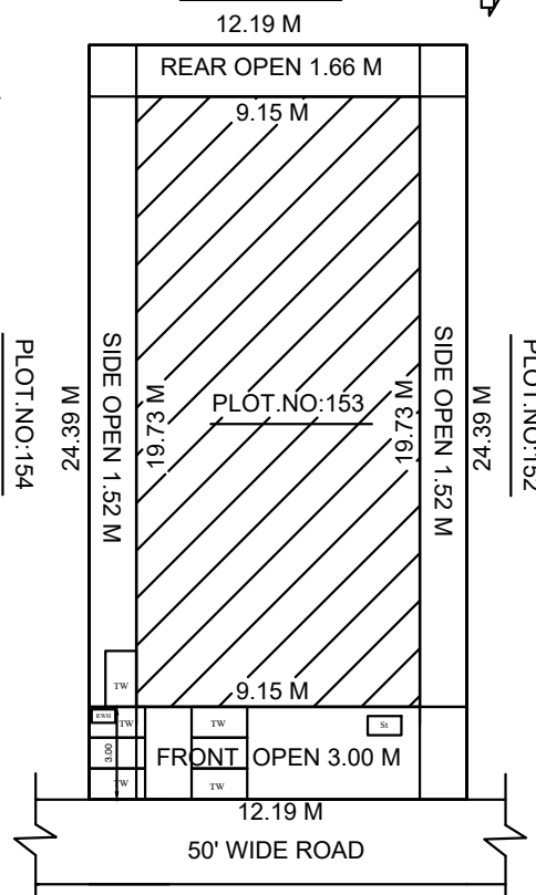
SITE PLAN
