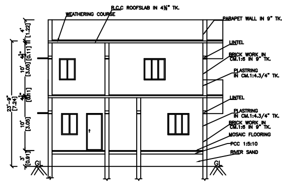
SECTION-"AB"
