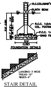
STAIR DETAIL
