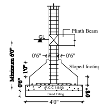
ISOLATED FOOTING / COLUMN DETAIL
