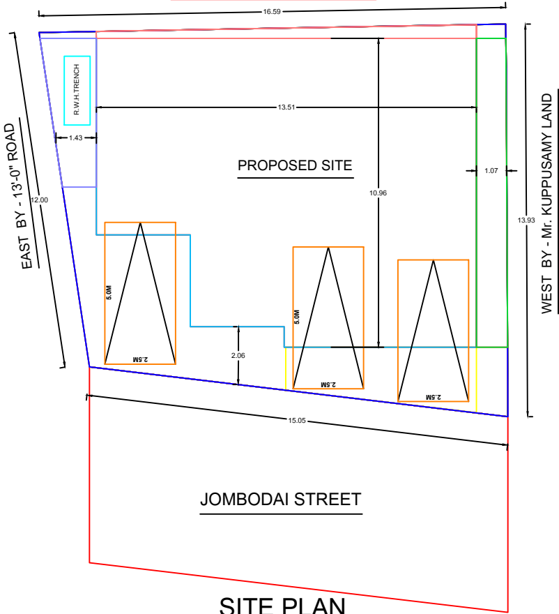
SITE PLAN
