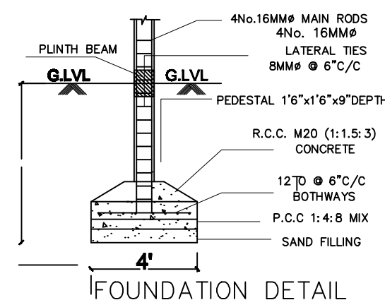
FOUNDATION DETAIL
