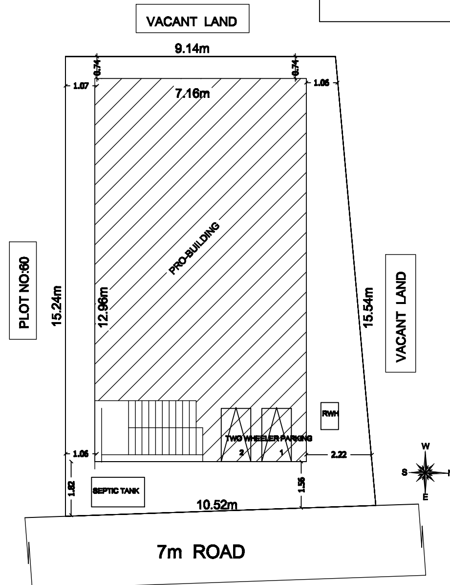
SITE PLAN
