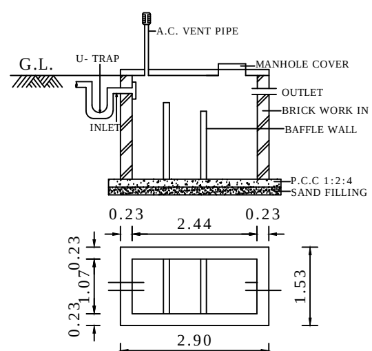
SEPTIC TANK DETAIL
