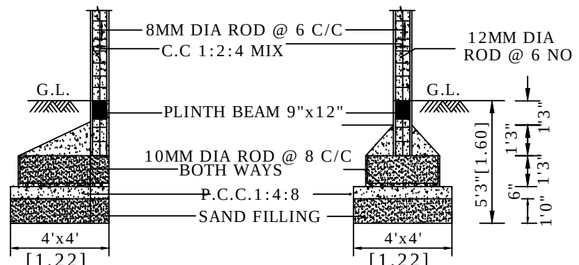
RUN THROUGH COLUMN FOUNDATION
