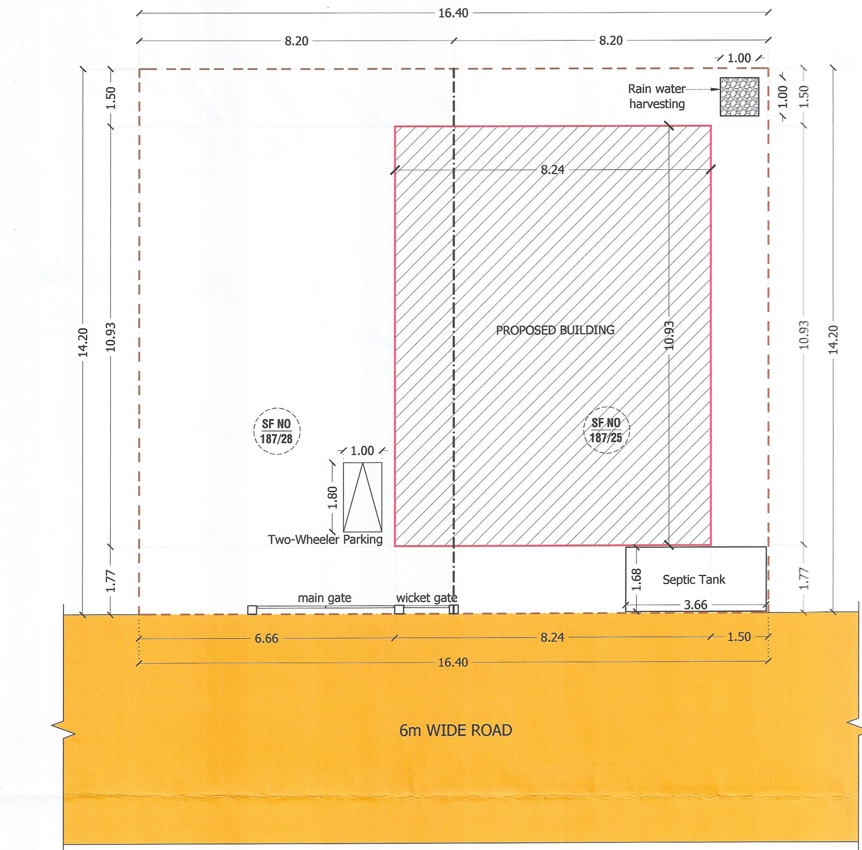
Site Plan
