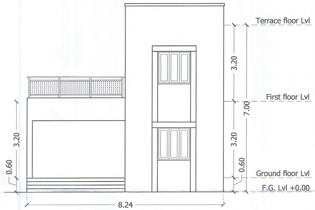
Front Elevation
