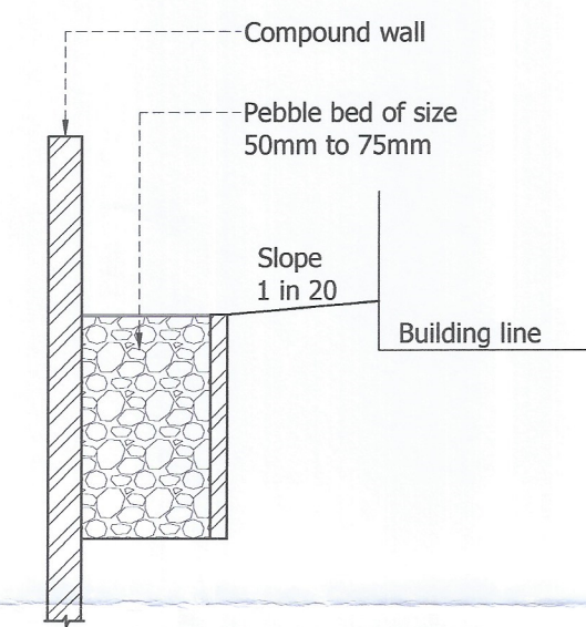
Rain water trench (NTS)
