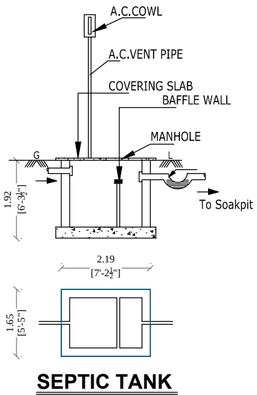
SEPTIC TANK
