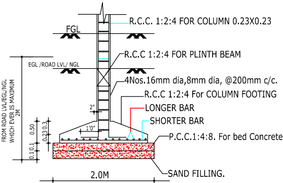
FOUNDATION DETAIL
