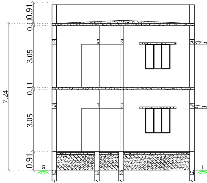
SECTION ON "SC"
