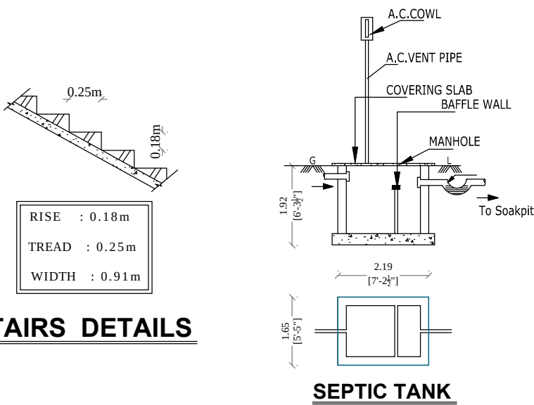
SEPTIC TANK
