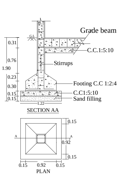
FOUNDATION DETAILS
