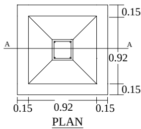
FOUNDATION DETAILS
