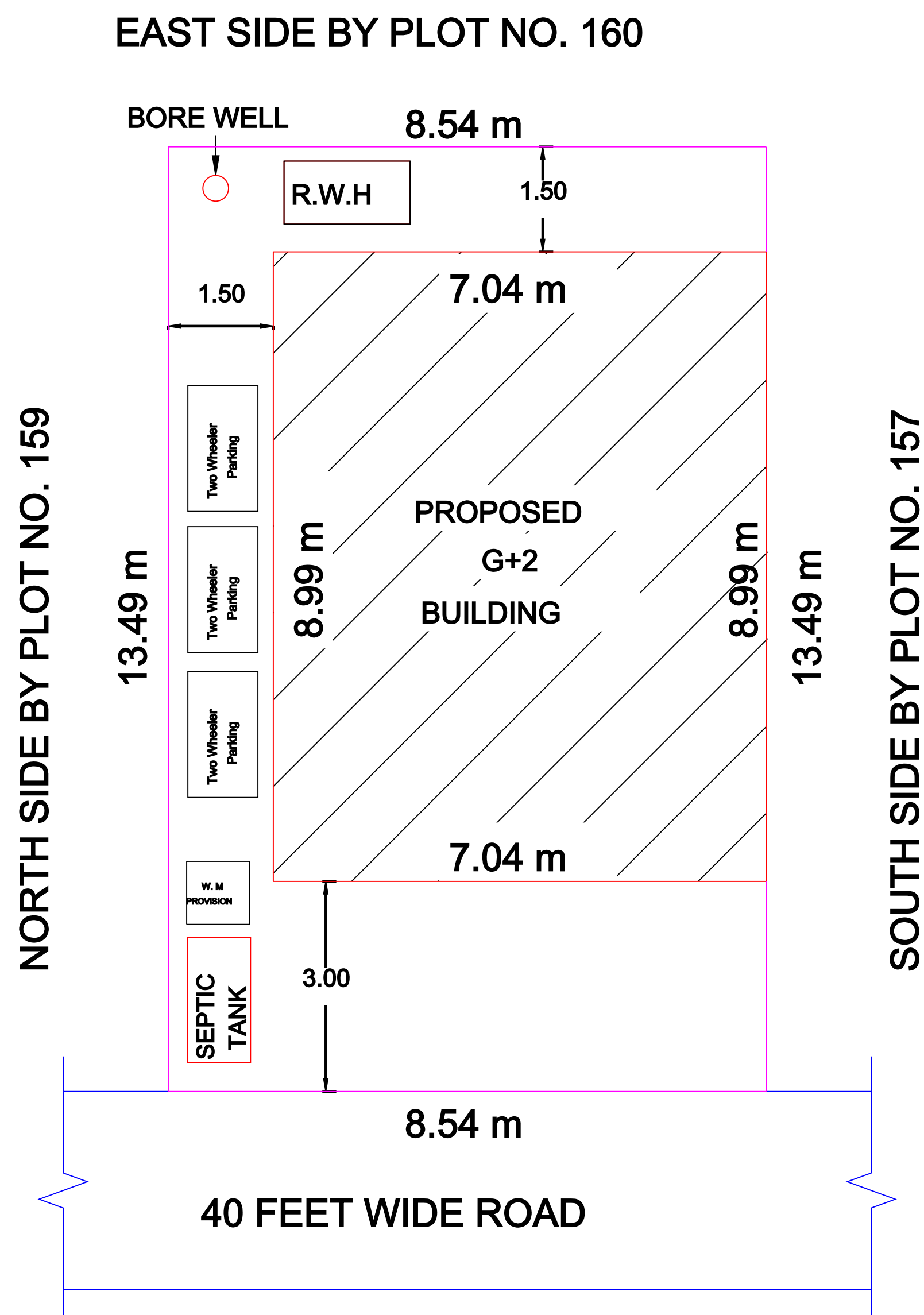
SITE PLAN
