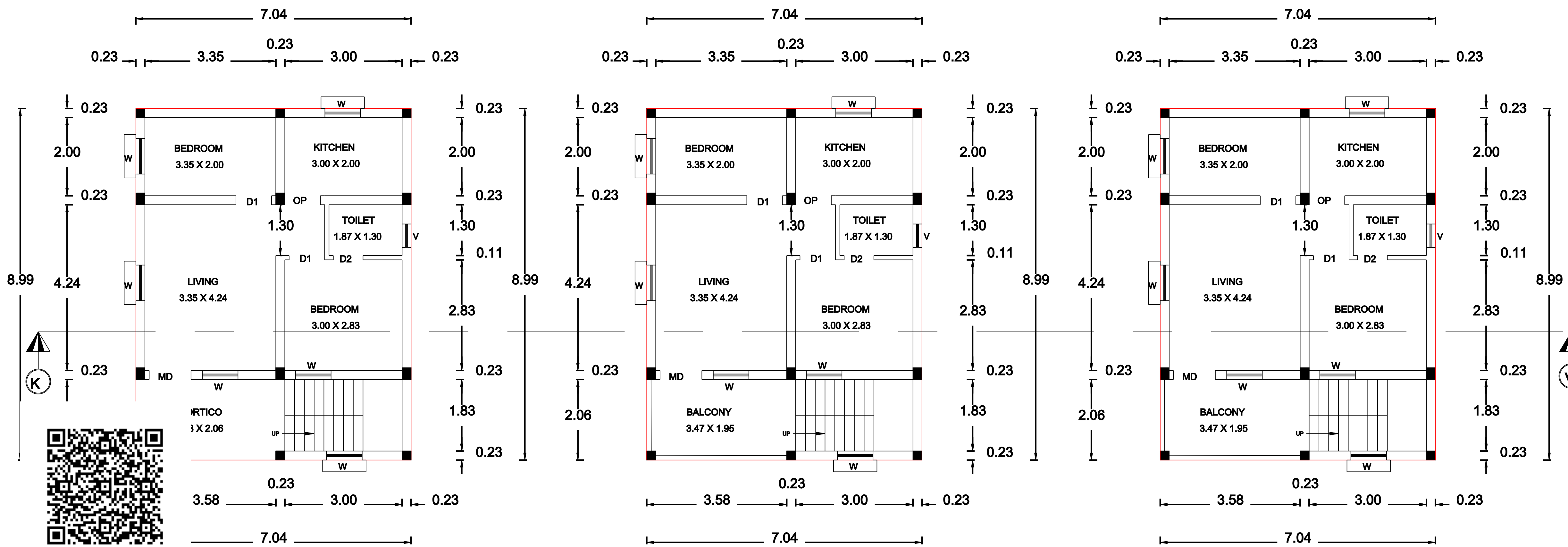
PRO. GROUND FLOOR PLAN
