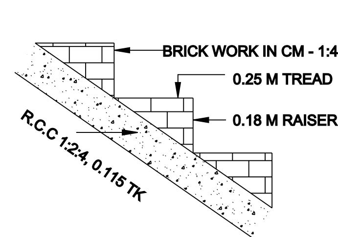
STAIR CASE DETAILS (SCALE 1 : 1)
