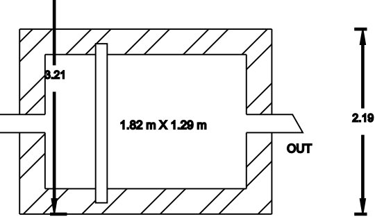
SEPTIC TANK (Scale 1 : 1)
