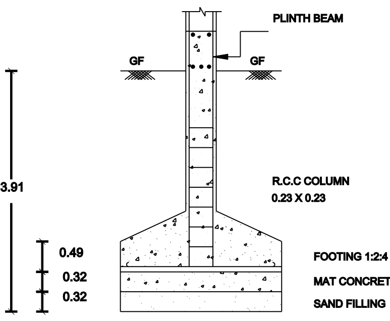
FOUNDATION DETAILS (SCALE 1 : 1)
