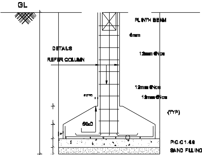
FOUNDATION DETAILS
