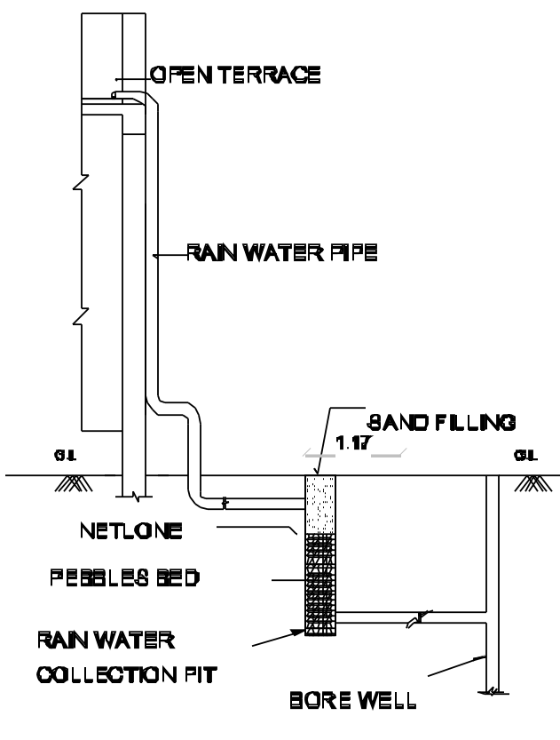
RAIN WATER HARVESTING SYSTEM
