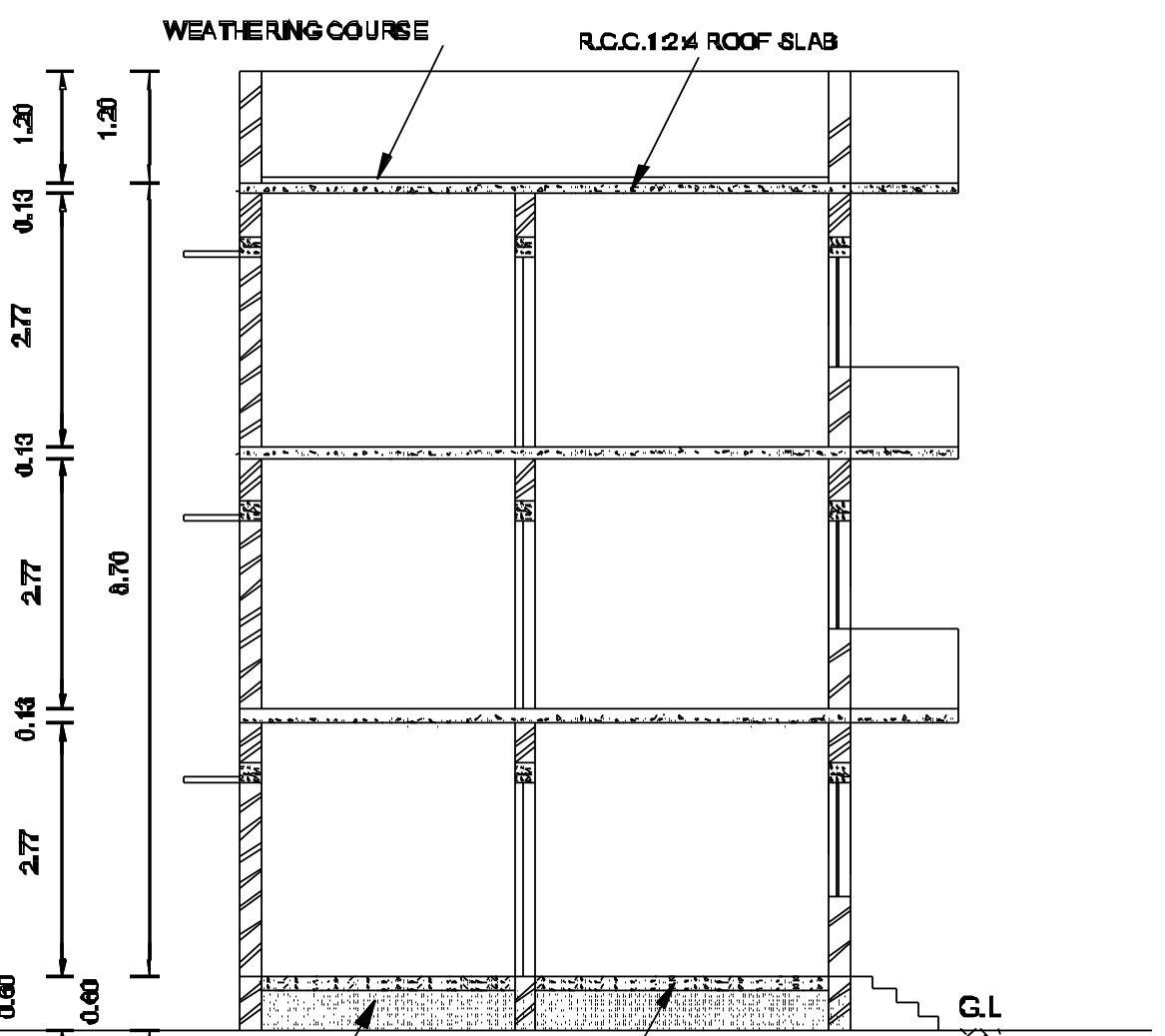
SECTION ON "MS"
