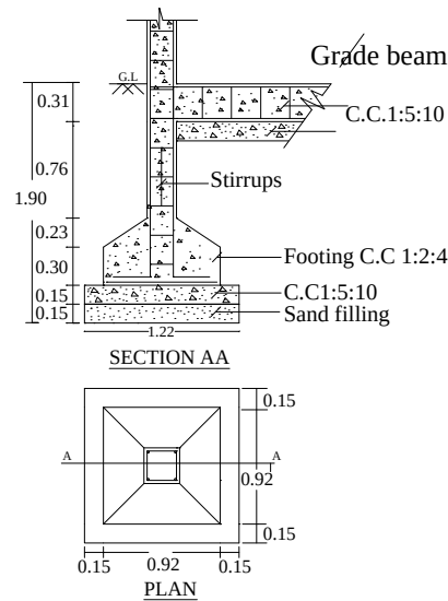
FOUNDATION DETAILS
