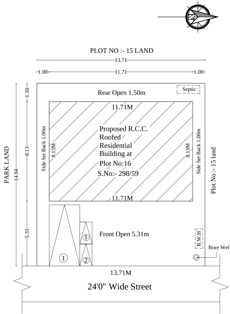
SITE PLAN
