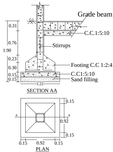
FOUNDATION DETAILS
