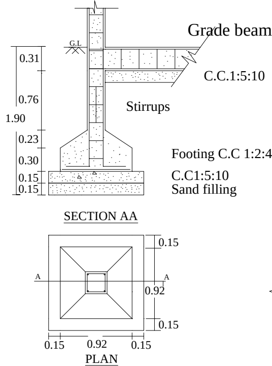
FOUNDATION DETAILS
