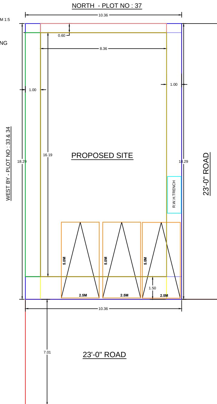
SITE PLAN
