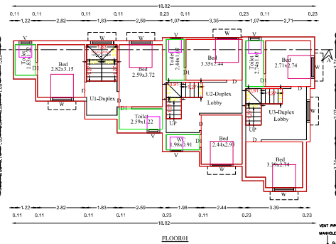
FLOOR PLAN
