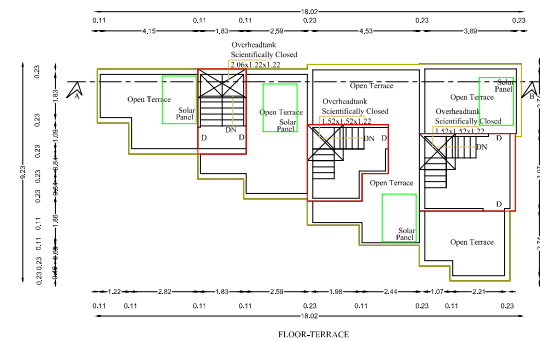
FLOOR TERRACE
