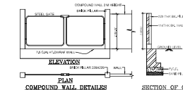
PLAN COMPOUND WALL DETAILS
