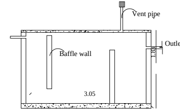
SEPTIC TANK DETAILS Size: 3.05 x 1.83 SCALE 1:100
