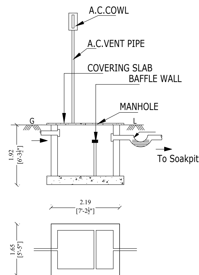
SEPTIC TANK
