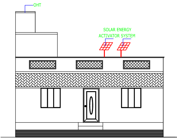
FRONT ELEVATION
