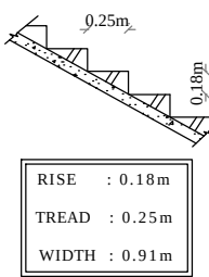
STAIRS DETAILS
