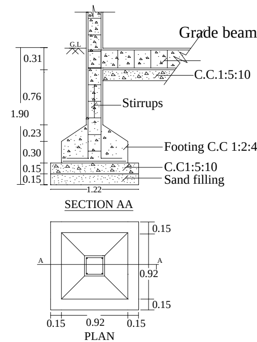
FOUNDATION DETAILS
