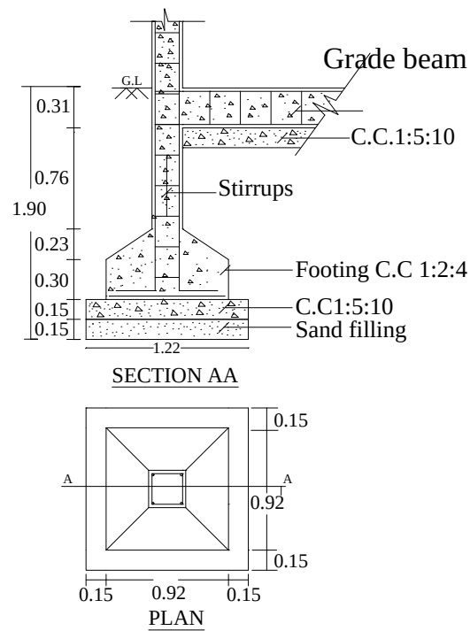
FOUNDATION DETAILS
