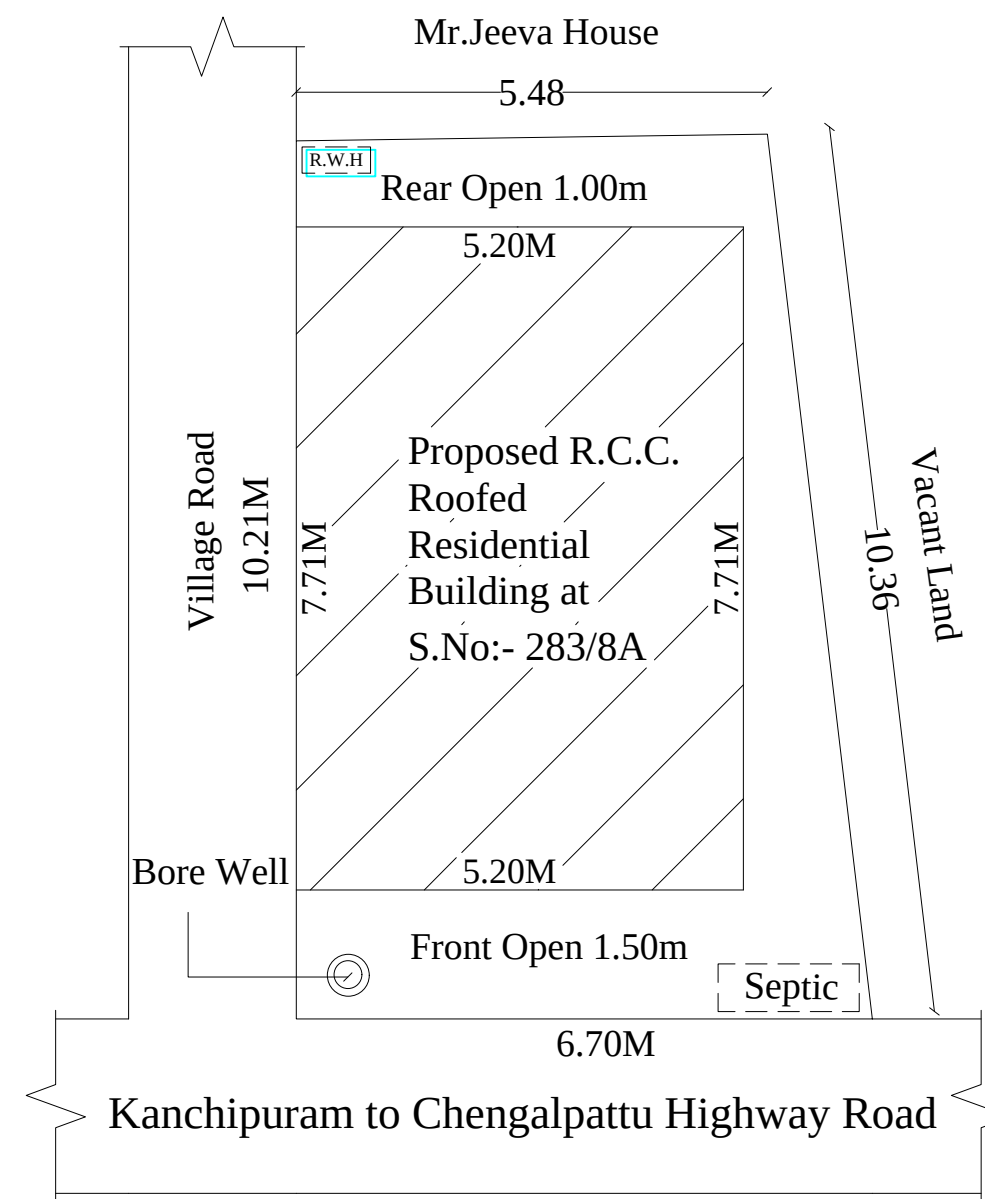
SITE PLAN
