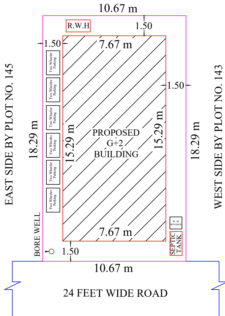
SITE PLAN
