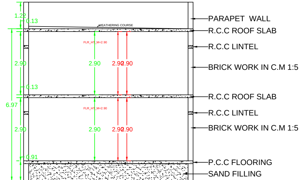
SECTION
