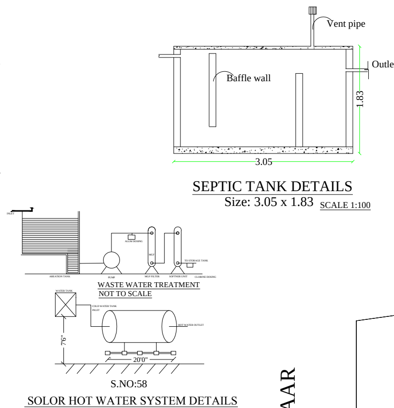
SOLOR HOT WATER SYSTEM DETAILS
