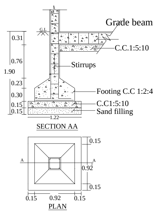
FOUNDATION DETAILS
