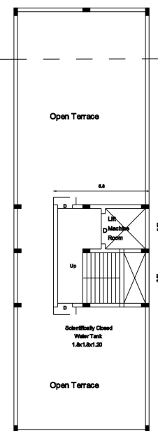
Terrace Floor Plan
