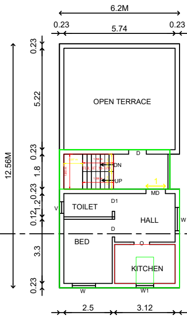
SECOND FLOOR PLAN 1:100
