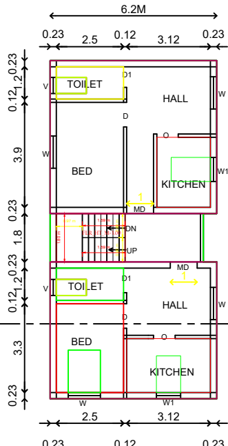
FIRST FLOOR PLAN 1:100
