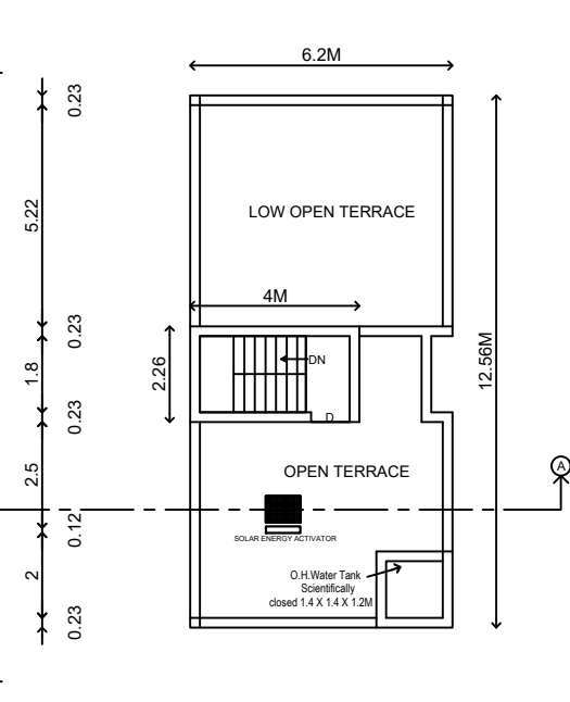
TERRACE FLOOR PLAN 1:100
