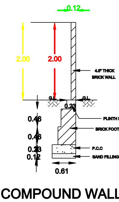
COMPOUND WALL
