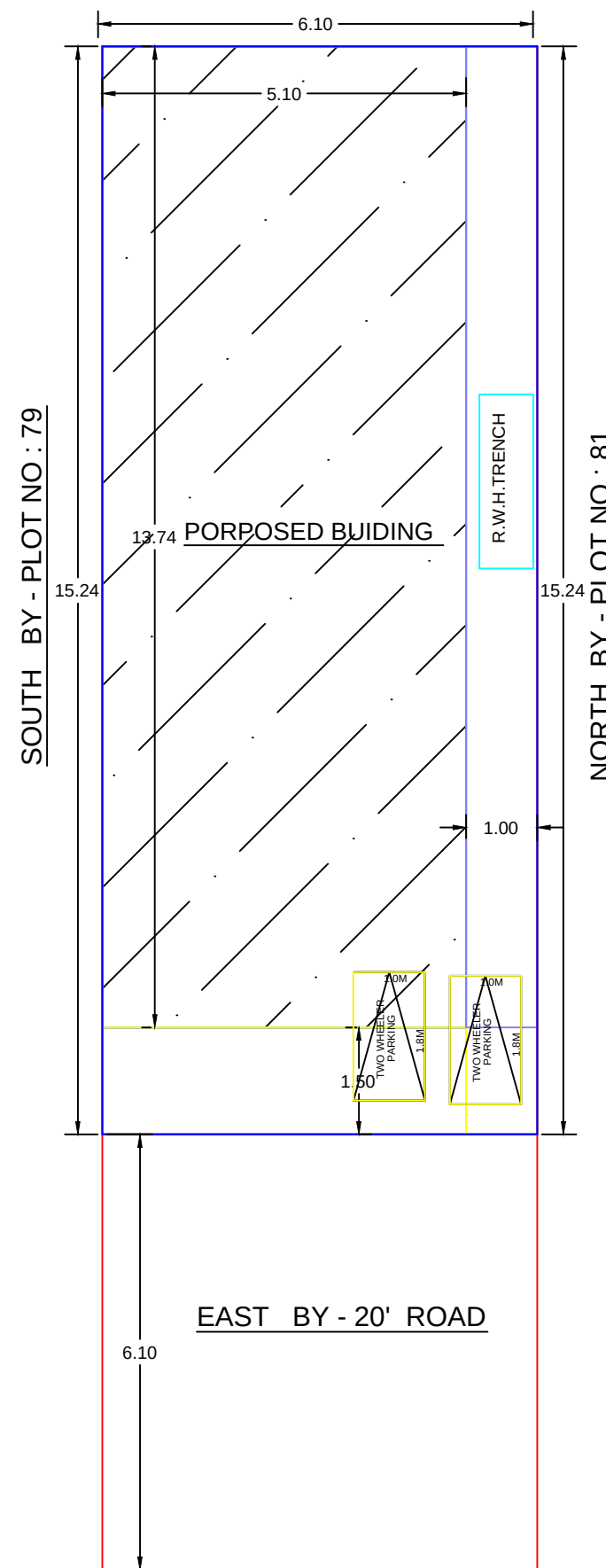
SITE PLAN
