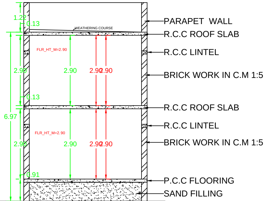
SECTION
