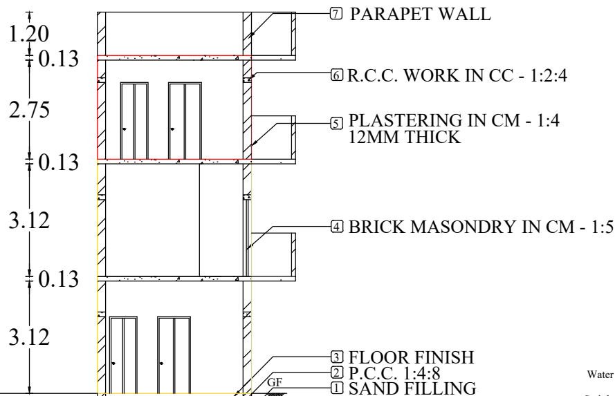
SECTION ON "KV"
