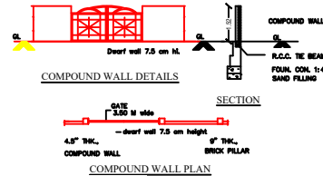
COMPOUND WALL PLAN
