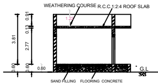
SECTION ON WALL
