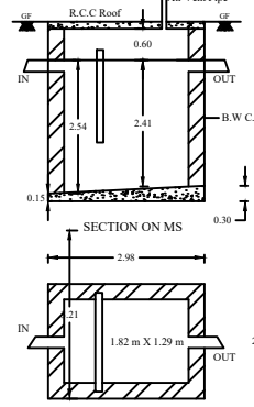
PLAN SEPTIC TANK (Scale 1 : 1)
