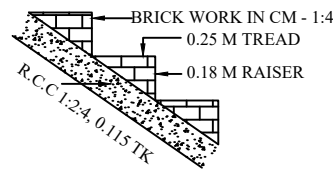
STAIR CASE DETAILS (SCALE 1 : 1)
