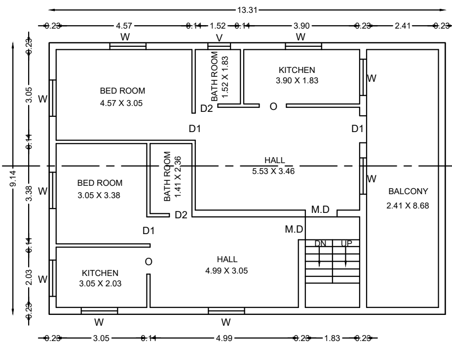
TYPICAL FLOOR PLAN (FIRST & SECOND FLOOR)
