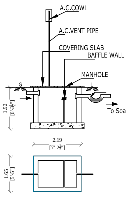
SEPTIC TANK
