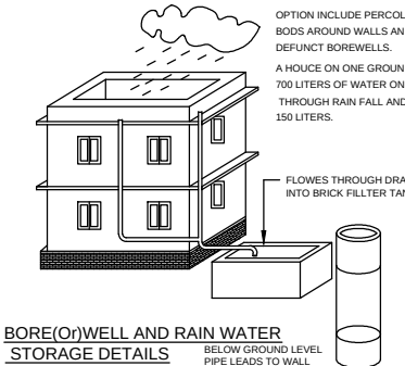
BORE(O)WELL AND RAIN WATER STORAGE DETAILS
