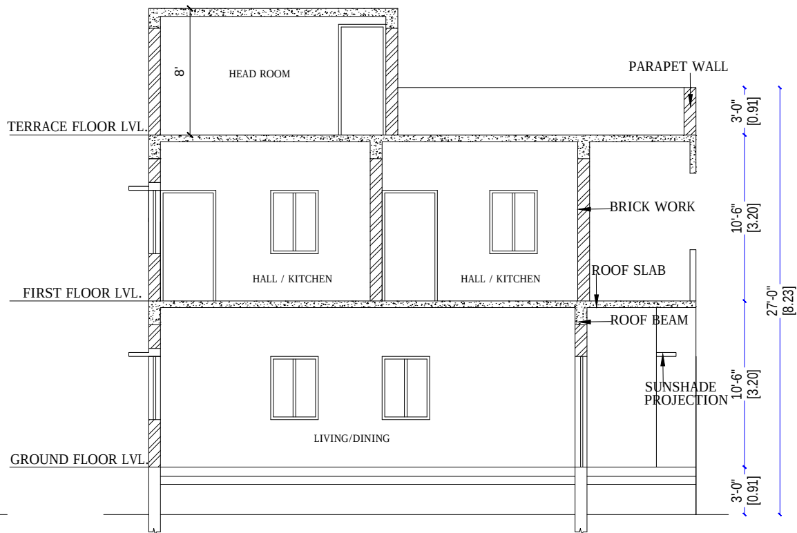
SECTION - AA
