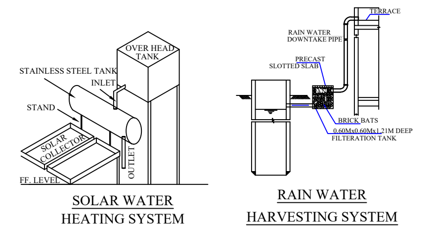
SOLAR WATER HEATING SYSTEM RAIN WATER HARVESTING SYSTEM
