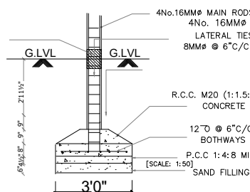
FOUNDATION DETAIL
