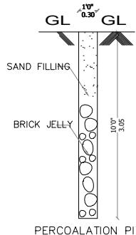
PERCOLATION PIT
