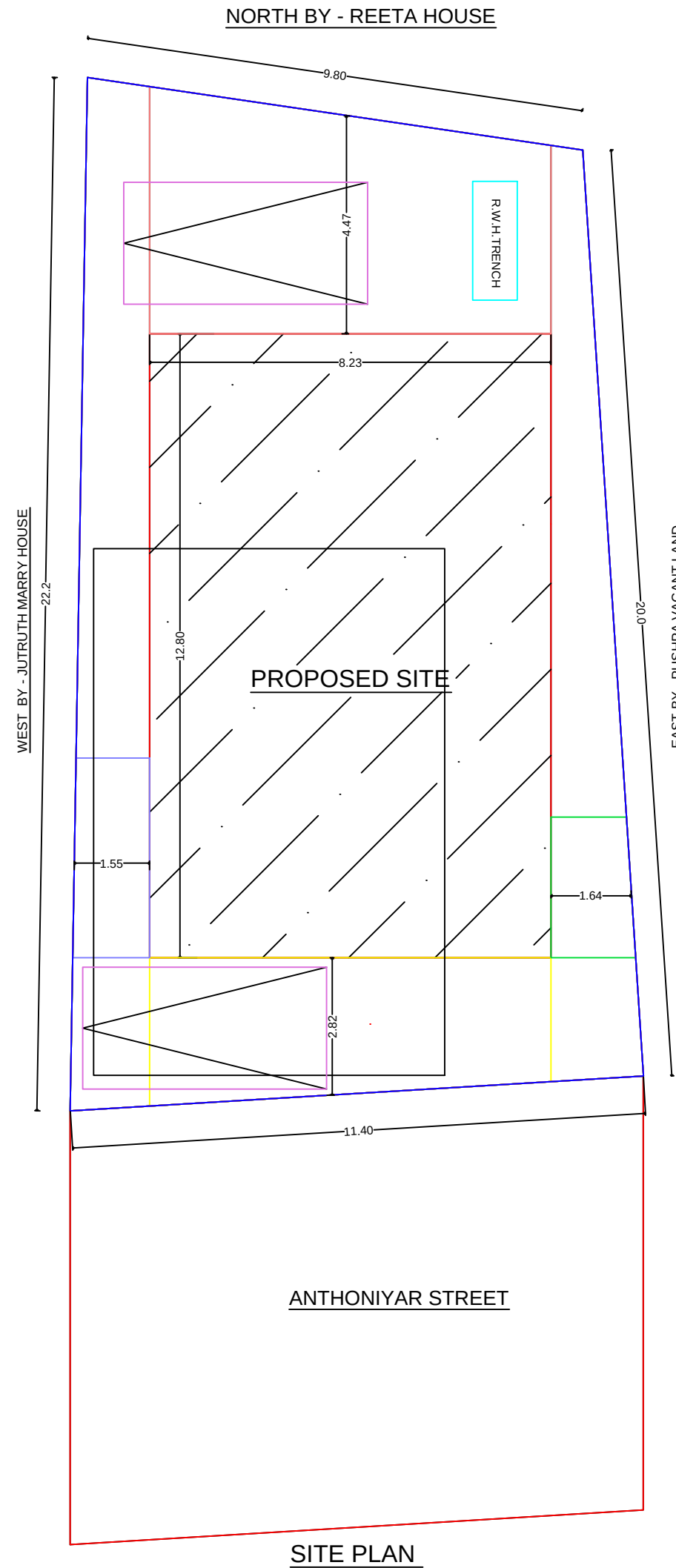
SITE PLAN
