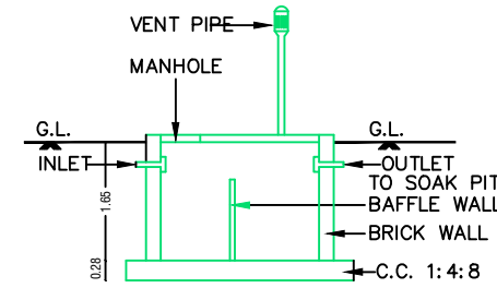
SECTION OF SEPT. TANK
