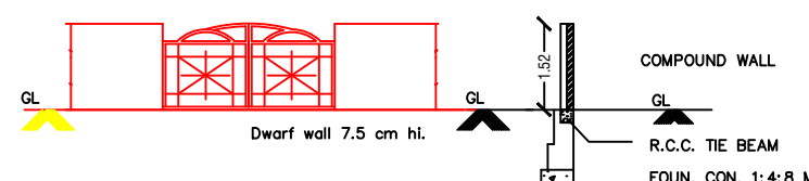
COMPOUND WALL DETAILS
