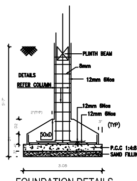
FOUNDATION DETAILS
