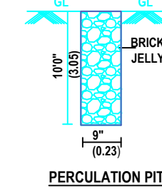
PERCOLATION PIT
