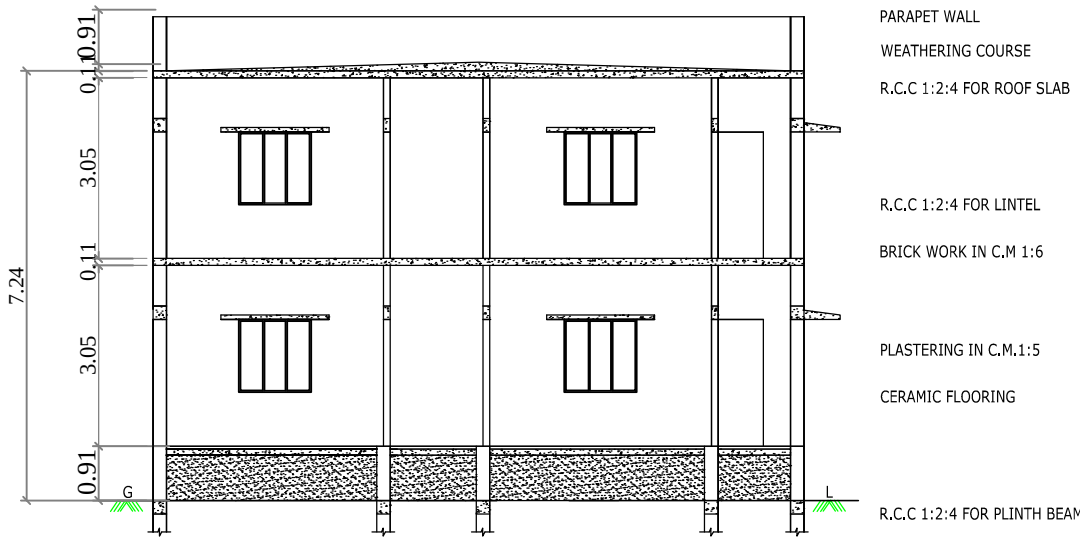
SECTION ON "SC"
