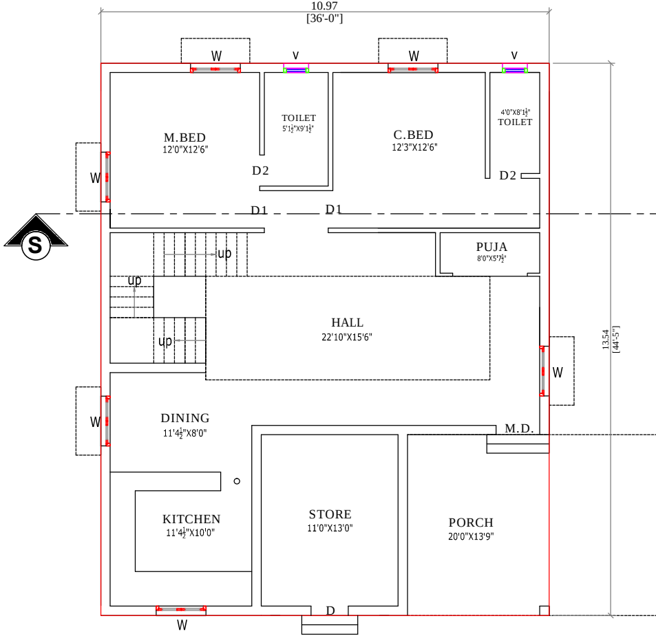
2 PLAN
