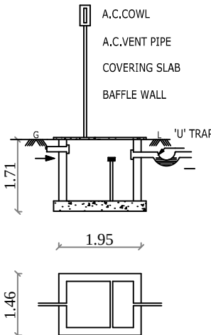
SEPTIC TANK
