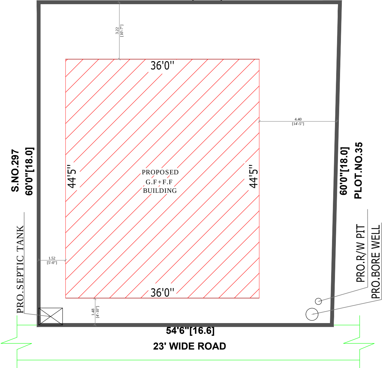
SITE PLAN SCALE: 1 INCH = 8 FEET
