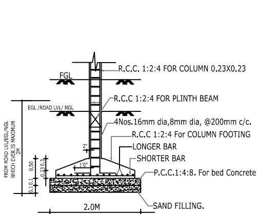
FOUNDATION DETAIL
