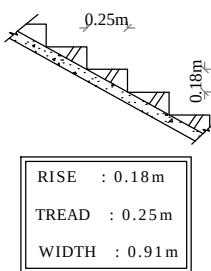
STAIRS DETAILS
