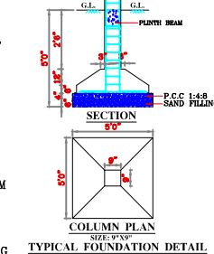
TYPICAL FOUNDATION DETAIL
