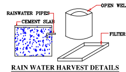
RAIN WATER HARVEST DETAILS
