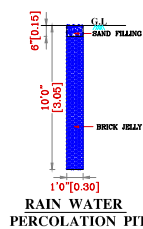
PERCOLATION PIT
