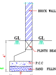
SECTION OF COMPOUND WALL
